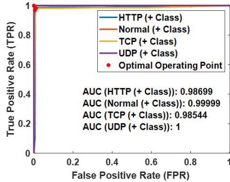
(f) ROC curve for CART.
