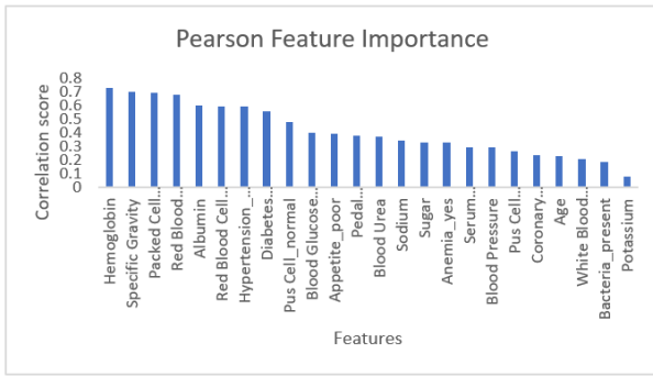
FIGURE 5. Feature ranking after applying Pearson correlation.
