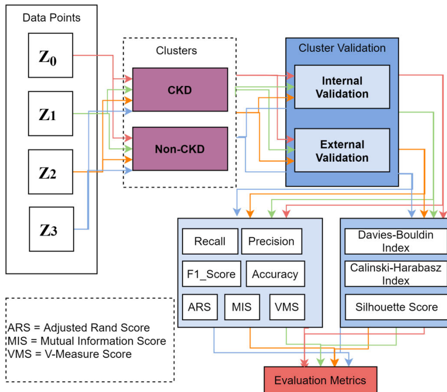
FIGURE 15. Cluster validation.
