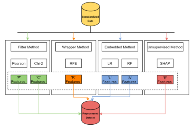
FIGURE 4. Feature reduction through feature elimination.
