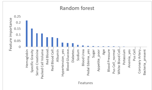
FIGURE 11. Feature ranking after applying random forest method.
