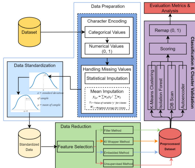
FIGURE 1. Workflow of the proposed method.
