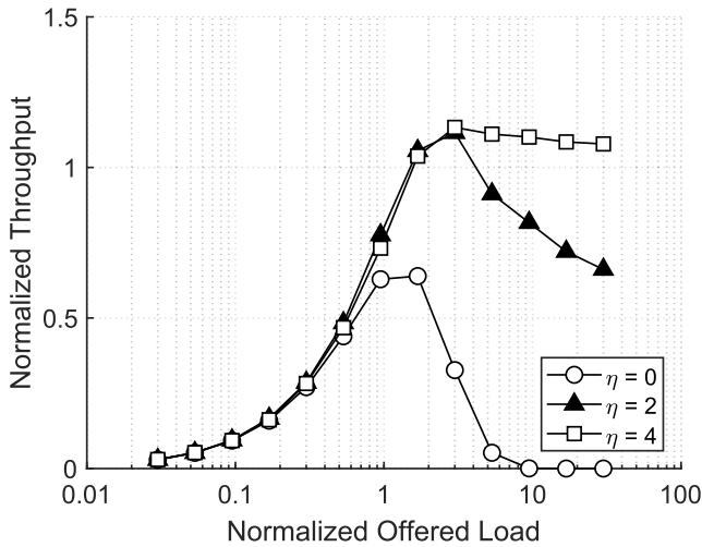
FIGURE 13. Performance of a LoRa cell with single LoRaSyNc GW and different values of path loss attenuation exponent \eta .
