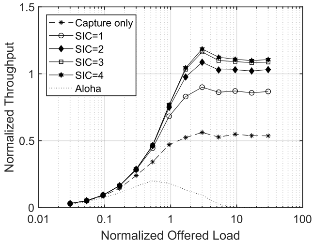
FIGURE 12. Performance of LoRaSyNc with increasing the number of SIC rounds (from 1 to 4), compared to a traditional GW (capture only) and the theoretical Aloha model. The improvement becomes negligible increasing the number of SIC iterations further.
