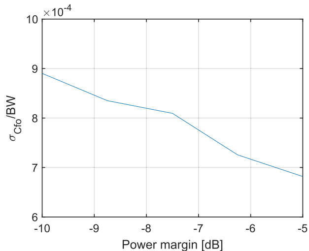
FIGURE 8. Standard deviation of the Cfo error estimate, using the following parameters: SF = 7, B = 125kHz, P threshold = -121 dBm.
