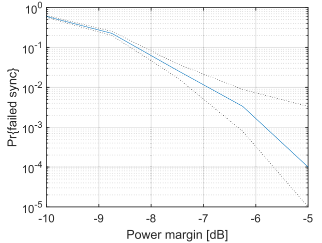
FIGURE 7. Probability of failing to detect a preamble, using the following parameters: SF = 7, B = 125kHz, P_{threshold} = -121 dBm. Dot lines limit the confidence interval.
