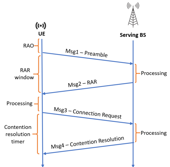
FIGURE 3. A graphical representation of the RA procedure.
