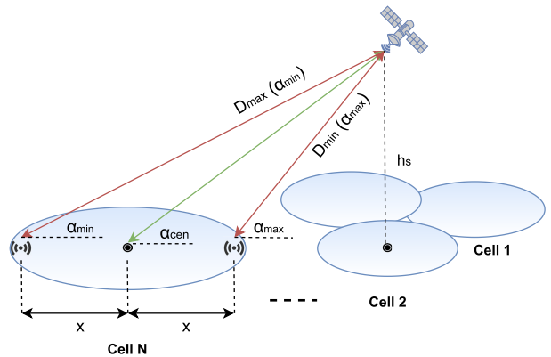
FIGURE 8. NTN system geometry.
