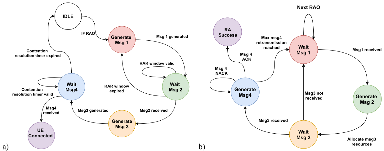
FIGURE 2. State machine representation during the RA procedure at: a) UE side and b) BS side.
