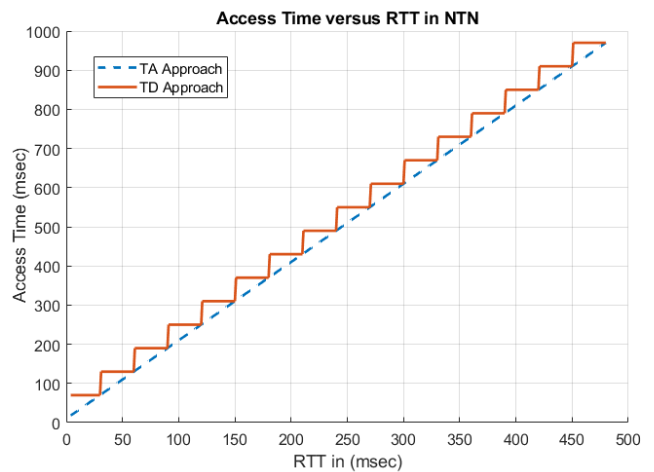
FIGURE 14. Single user access time (no collision).
