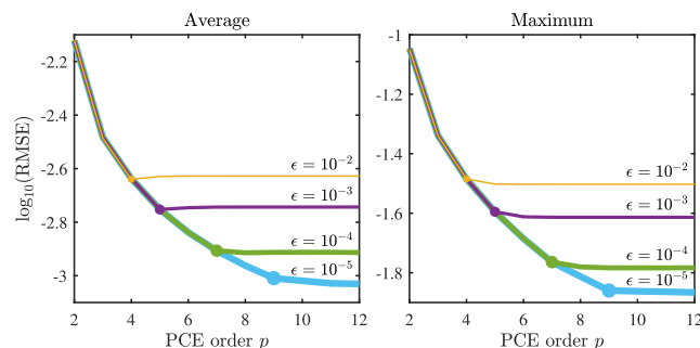
FIGURE 4. Average (left) and maximum (right) RMSE over frequency obtained with rational PCEs of various orders, applied in conjunction with PCA compression with different truncation thresholds. The dots mark the point at which the expansion order matches the number of principal components.
