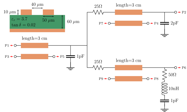
FIGURE 6. Schematic of the nine-port network with coupled microstrip lines [21], with port definition.
