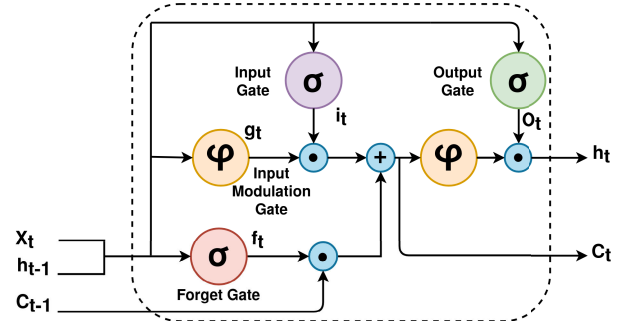
FIGURE 1. LSTM cell.
