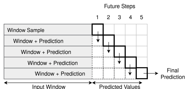
FIGURE 4. Rolling ARIMA example with the forecasting horizon of 5 steps.
