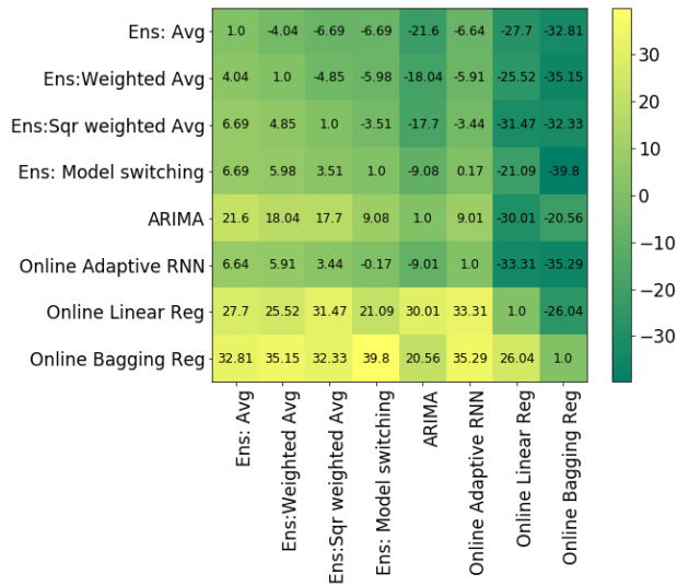
FIGURE 18. Diebold-Mariano test: DM values for house Low1.
