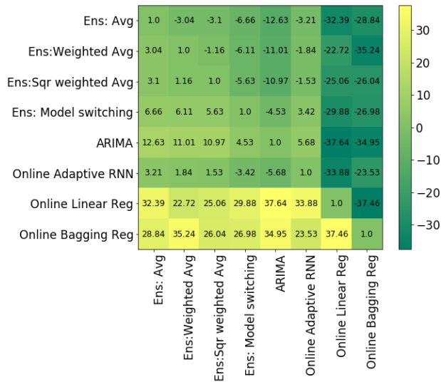
FIGURE 19. Diebold-Mariano test: DM values for house Low2.
