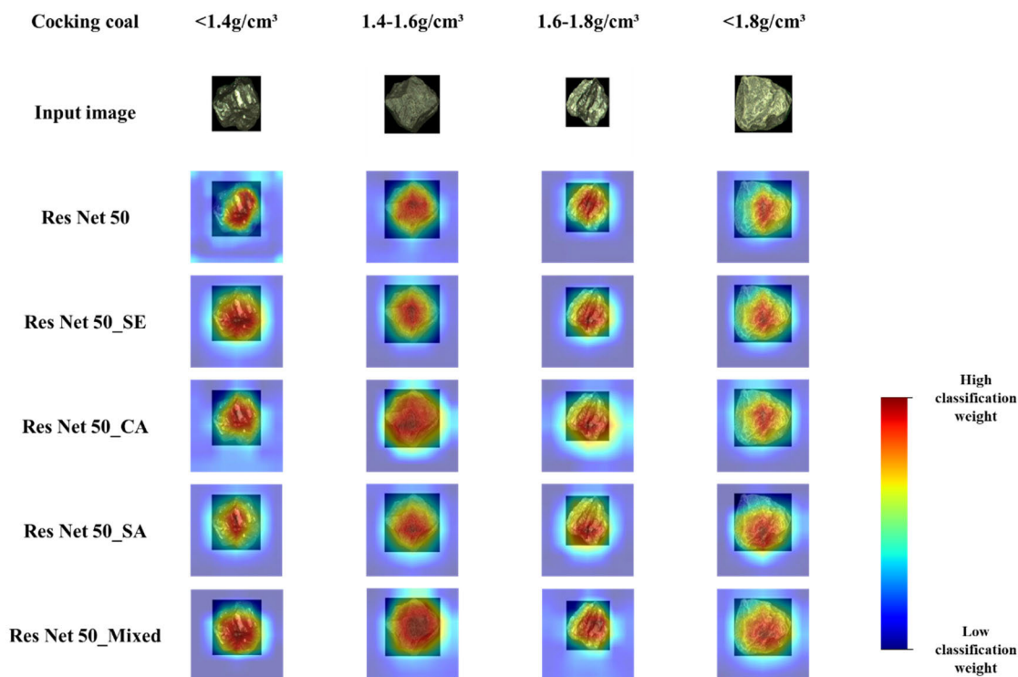
FIGURE 12. Grad-CAM maps of ResNet50 with different attention blocks for four-classes cocking coal image classification.
