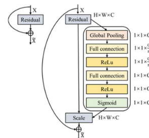
FIGURE 5. Squeeze and excitation block setting in ResNet.
