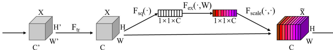
FIGURE 4. Squeeze and excitation block framework in CNNs, where H, W, and C are the dimension of the feature map, H is height, W is width, C is channel, F_{tr} is the convolution calculation, F_{sq} is the Squeeze operation, F_{ex} is the Excitation operation, F_{scale} is the Reweight operation, \tilde{X} is the feature map after attention.
