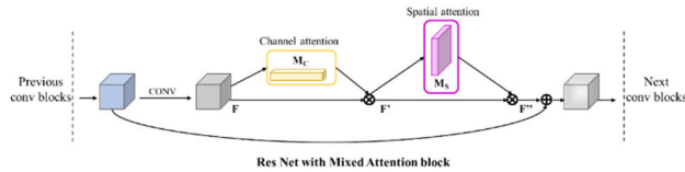
FIGURE 8. Mixed attention block setting in ResNet.
