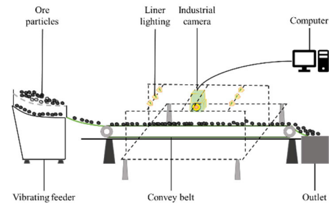
FIGURE 9. Ore particle image acquisition system consisted of vibrating feeder, conveyer belt, liner lighting, industrial camera, computer and outlet.
