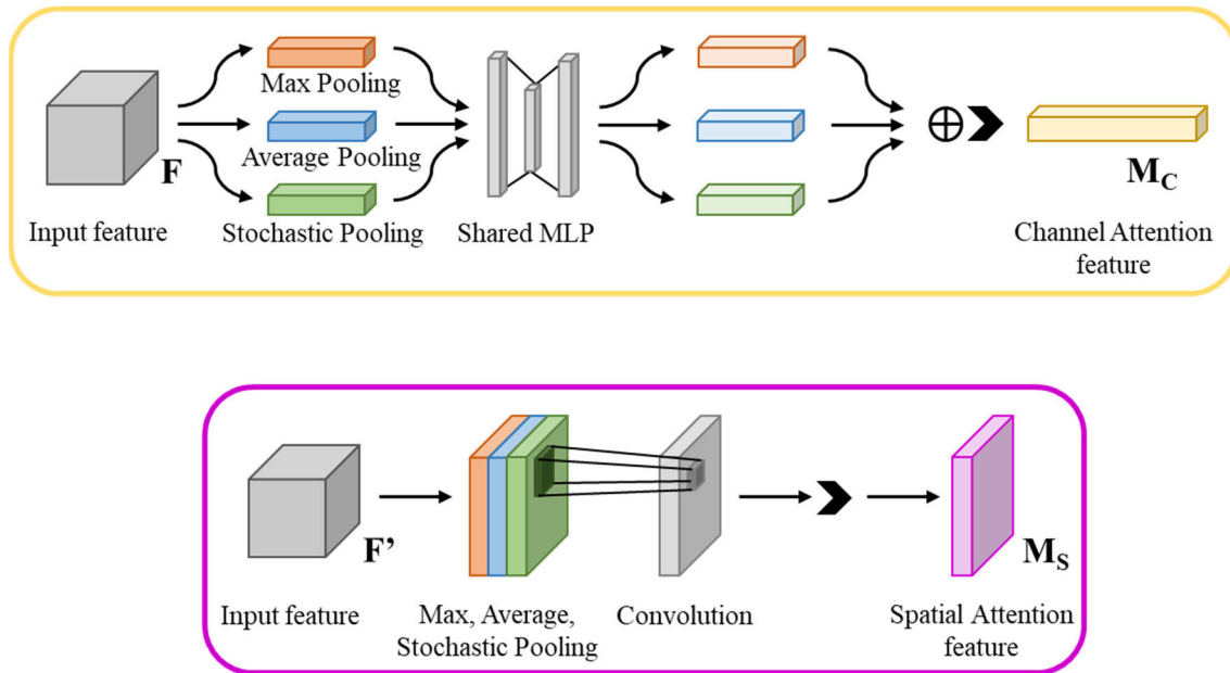
FIGURE 6. Channel attention block and spatial attention block framework.
