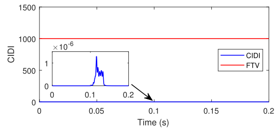
FIGURE 14. Current islanding detection indicator during SPP outage event.
