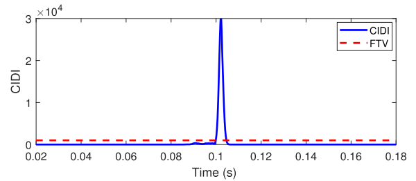
FIGURE 18. CIDI computed in real time scenario for Islanding event in the presence of solar power and wind power generation.
