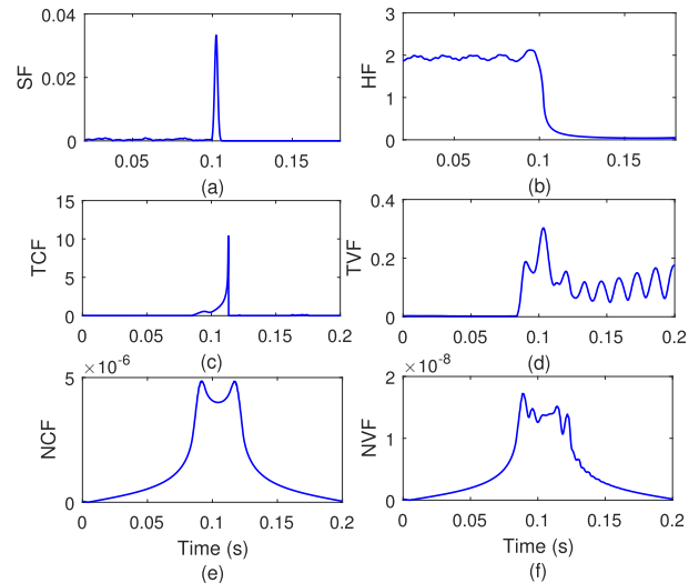
FIGURE 3. Identification of islanding scenario with availability of both WPP and SPP (a) Stockwell factor (b) Hilbert factor (c) current THD factor (d) voltage THD factor (e) negative sequence current factor (f) negative sequence voltage factor.
