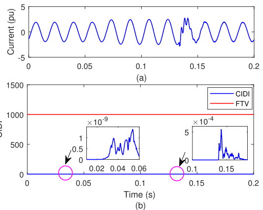
FIGURE 11. Identification of capacitor bank operation event (a) current signal associated to phase-A (b) current islanding detection indicator.
