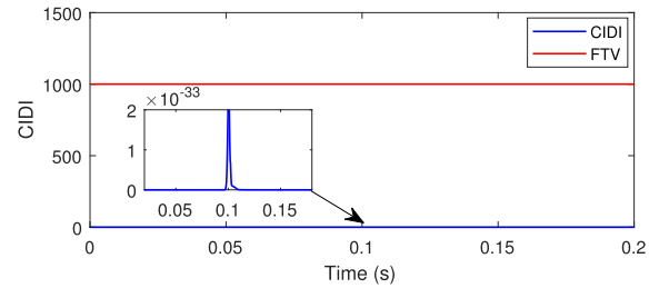
FIGURE 10. Current islanding detection indicator during LL fault event.
