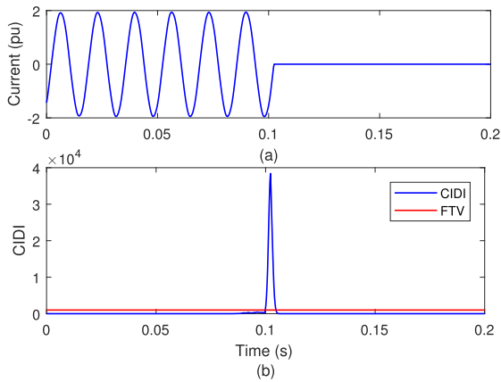
FIGURE 4. Identification of islanding event with availability of generation from both WPP and SPP (a) current associated to phase-A (b) current islanding detection indicator.
