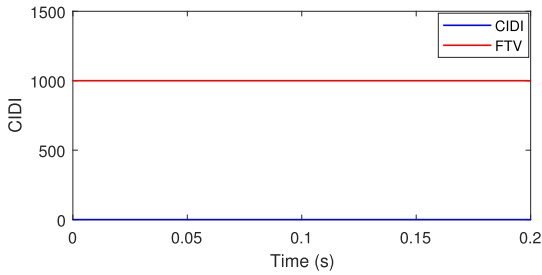
FIGURE 12. Current islanding detection indicator during inductive load operation event.
