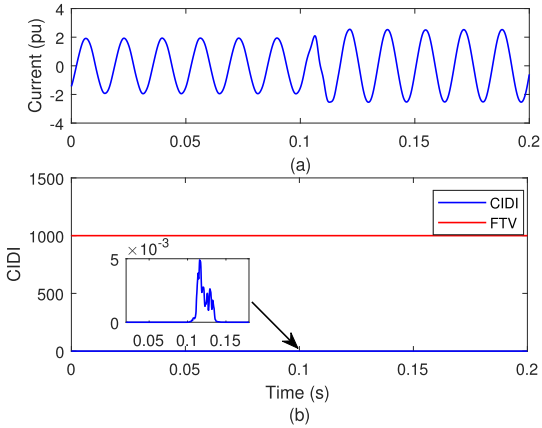
FIGURE 13. Identification of capacitor WPP outage event (a) current signal associated to phase-A (b) current islanding detection indicator.
