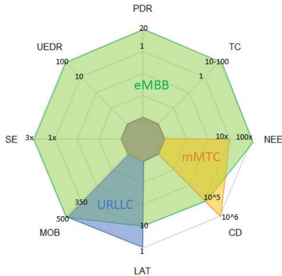
FIGURE 1. Standardized types of 5G networks IMT-2020 (5th generation) according to ITU-R M.2083 [11].
