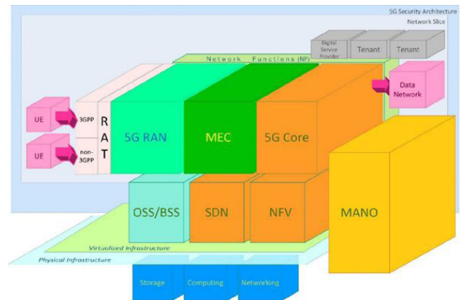
FIGURE 2. Schematic diagram of the 5G MEC network architecture, according to ENISA [152].
