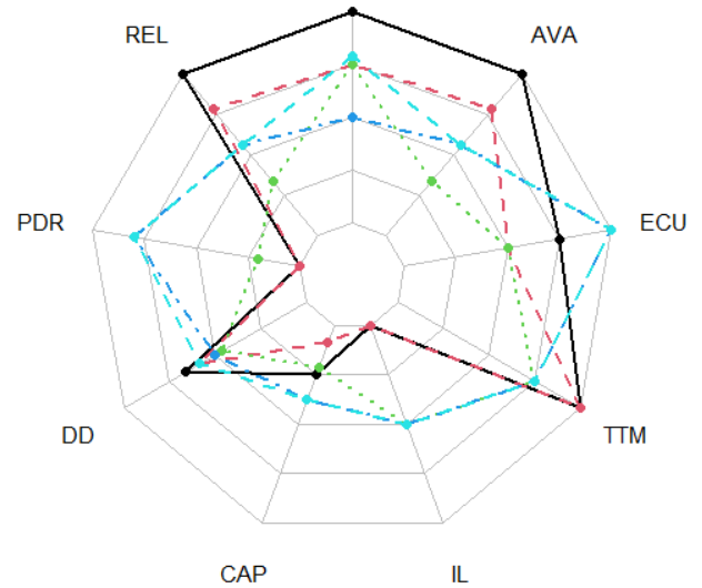
FIGURE 5. Requirements for use cases in the manufacturing industry ((1) black: Robotic control; (2) red: Automated guided vehicle; green: (3) Video surveillance; (4) blue: Quality check; (5) light blue: Augmented reality).
