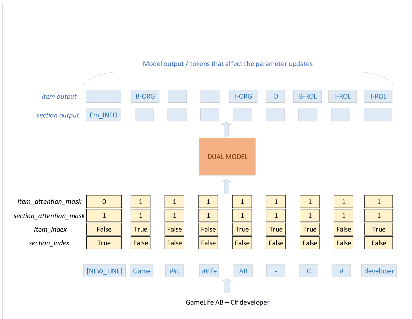
FIGURE 1. Dual model: example of one pass.
