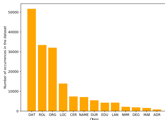
FIGURE 4. Item level: category frequencies in the annotated set (excluding 0 which appears 1 613 123 times).
