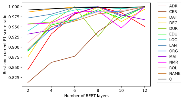
FIGURE 11. Influence of the number of BERT layers before the last linear layer to the macro-average F1 scores of the individual classes of the dual model (item level).
