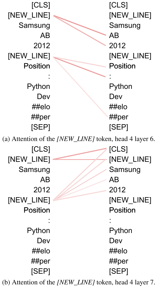
FIGURE 13. Different role of the [NEW_LINE] token inside different heads of the dual model. Visualization obtained using [22].
