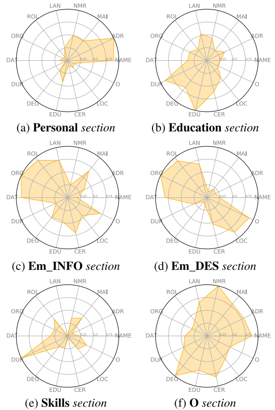
FIGURE 14. Item level classes with the largest attention values inside each head of all layers of the dual model, counted for all [NEW_LINE] tokens during section level prediction.
