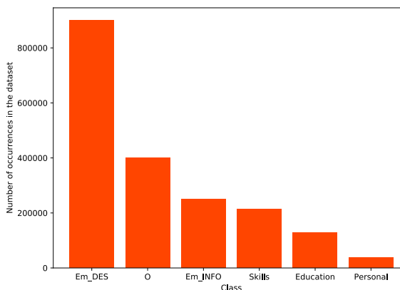
FIGURE 5. Section level: category frequencies in the annotated set.
