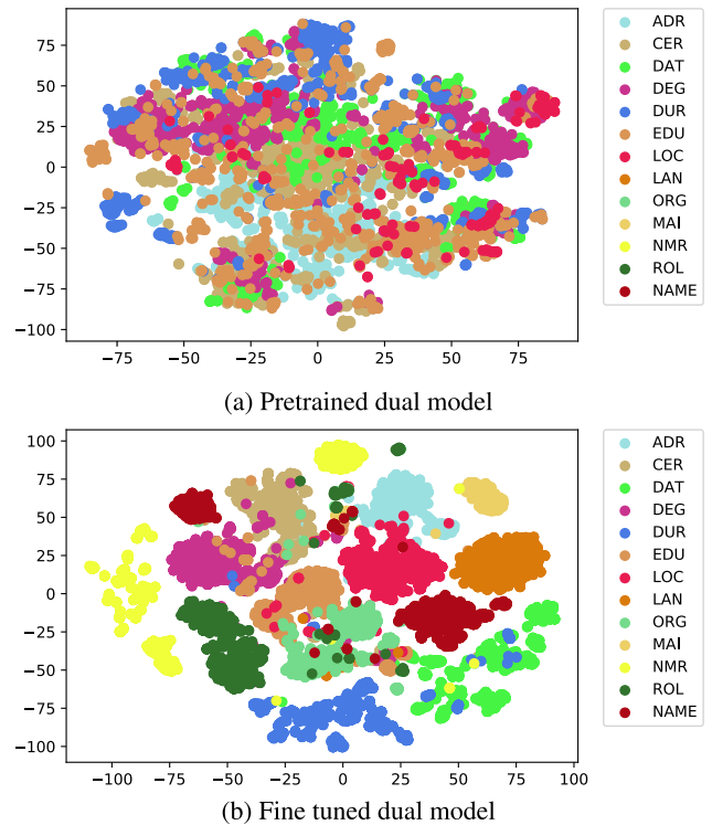
FIGURE 16. Vector representations of the pretrained and fine tuned dual model for item level tokens inside the validation set for each class, reduced to two dimensions using t-SNE algorithm.
