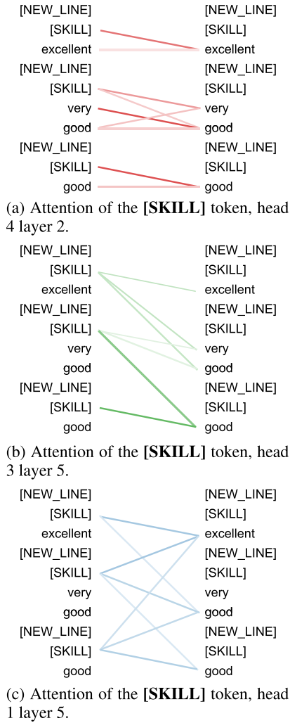
FIGURE 15. Different roles of the [SKILL] tokens inside different skill assessment models. Visualization obtained using [22].
