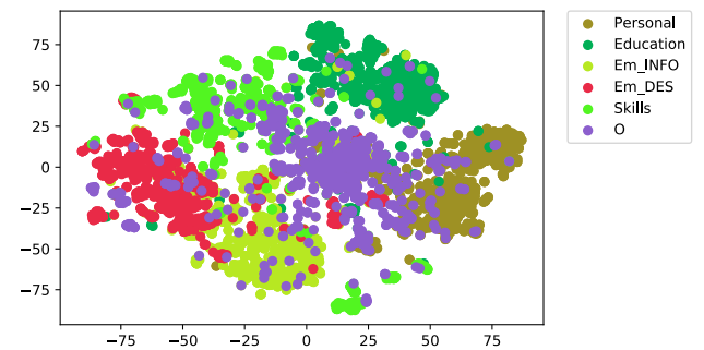
FIGURE 17. Vector representations of the fine tuned dual model [NEW_LINE] tokens of the section level inside the validation set for each class, reduced to two dimensions using t-SNE algorithm.
