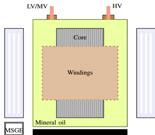
FIGURE 1. Representation of oil-immersed power transformer cross-section.
