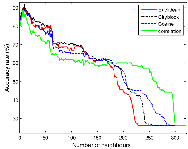
FIGURE 3. Impact of input vector “type 1” and number of neighbors on the classification performance (accuracy rate).
