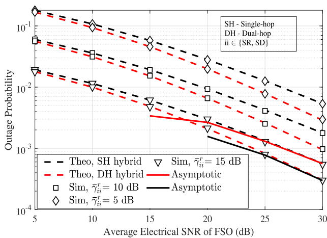
FIGURE 10. Outage probability vs Average electrical SNR of FSO link for different values of average SNR of RF for uplink scenario.
