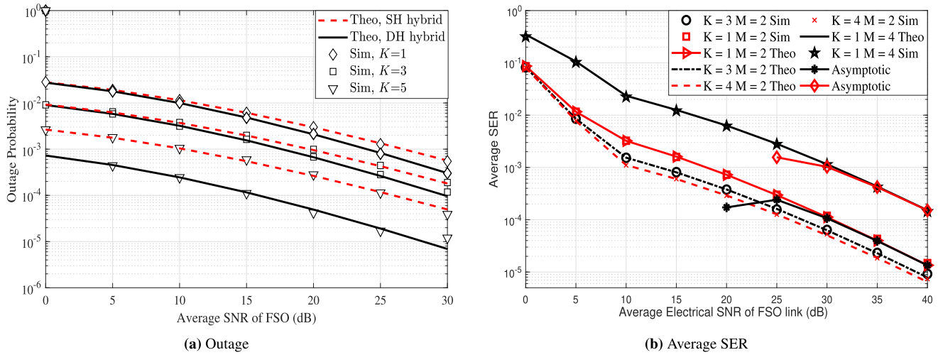
FIGURE 6. System performance parameters vs Average electrical SNR of FSO link for varying K for uplink scenario.
