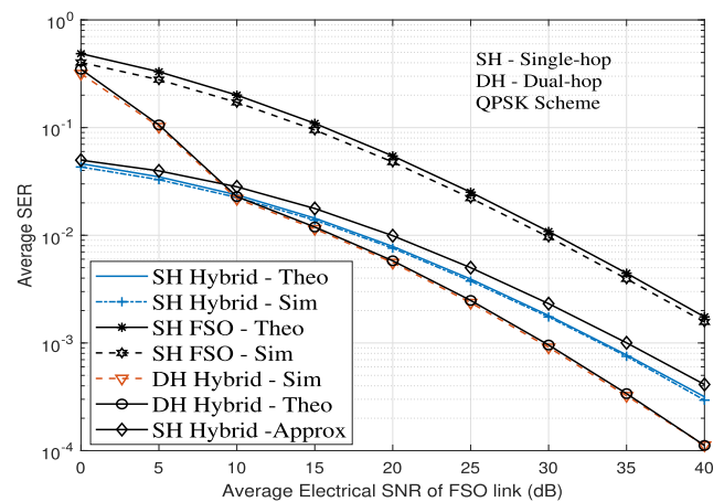
FIGURE 2. Performance comparison of theoretical and simulated average SER.
