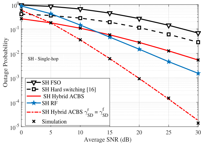
(a) Outage comparison of different switching schemes and system models
