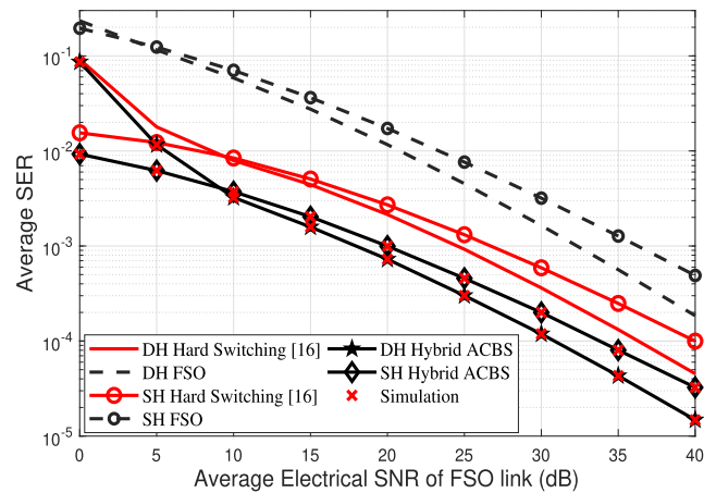
(b) SER comparison of different switching schemes and system models
