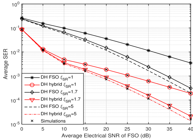
FIGURE 9. Average SER performance of dual-hop FSO and hybrid systems for different values of pointing error severity parameter \xi_{SR} .
