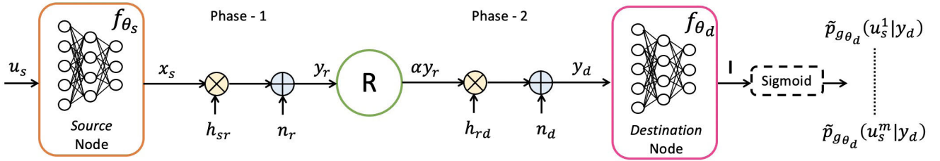
FIGURE 3. Bit-wise autoencoder (BWAEE) framework for amplify-and-forward relay networks.
