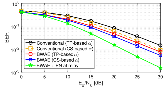
(b) Bit-wise AE with power normalization (PN) at relay node.
