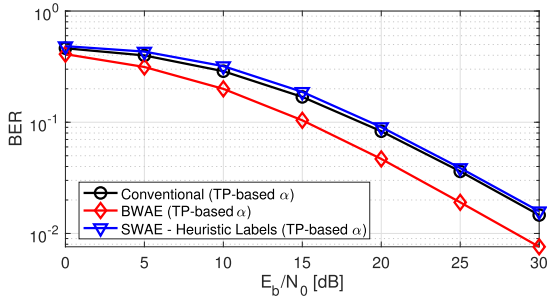
(a) Conventional versus Proposed AE Frameworks.
