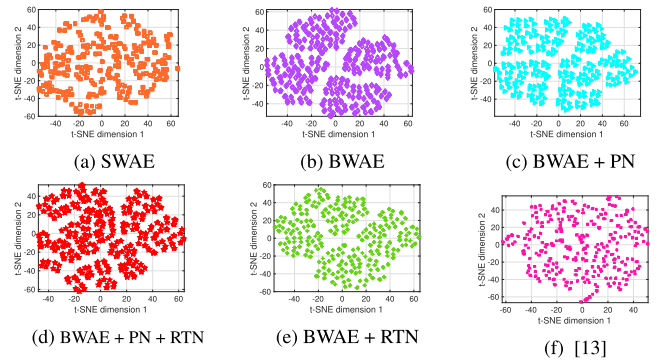
FIGURE 8. t-SNE representation in 2 dimensions.
