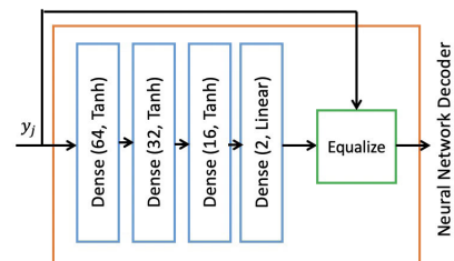
FIGURE 9. Radio transformer network (RTN).
