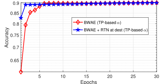
(d) Convergence of BWAE in presence of RTN in decoders.
