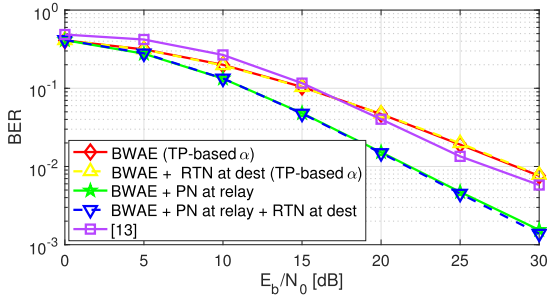
(c) RTN network in decoders and comparison with [13].
