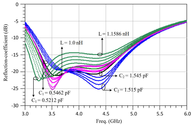
FIGURE 10. Effect on the reflection-coefficient response by the T-matching network parameters.
