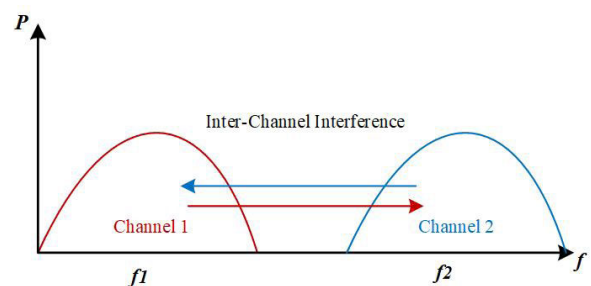
FIGURE 4. Inter-channel interference.
