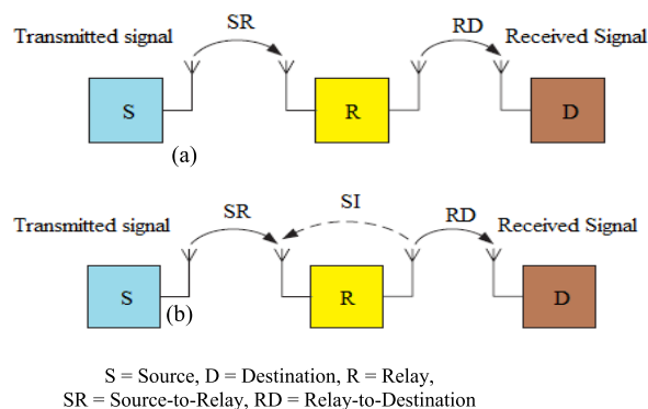
FIGURE 9. (a) Co-tier Ideal FDR (b) FDR with SI.
