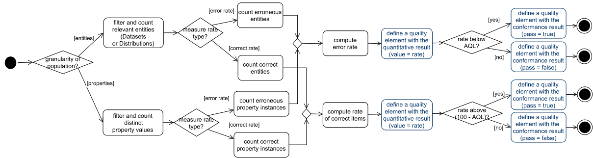
FIGURE 6. Workflow for reporting quality elements associated with automated measures.
