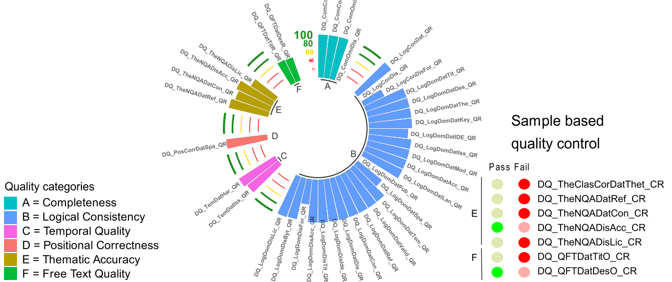
FIGURE 12. ISO 19157 dashboard summarizing the results shown in Tables 6, 7, and 8 (the labels correspond with the quality element identifiers in these tables).
