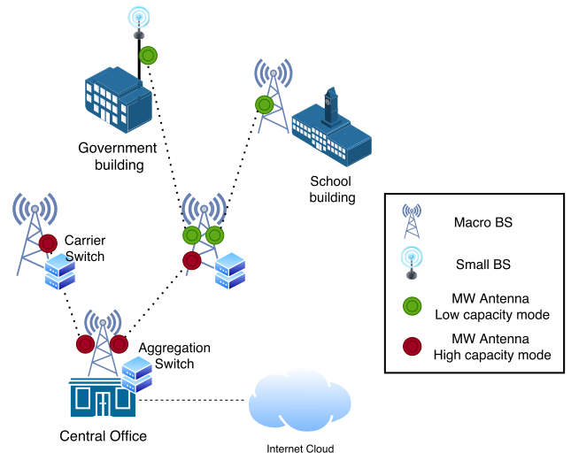
FIGURE 3. Wireless transport architecture for rural and remote areas.
