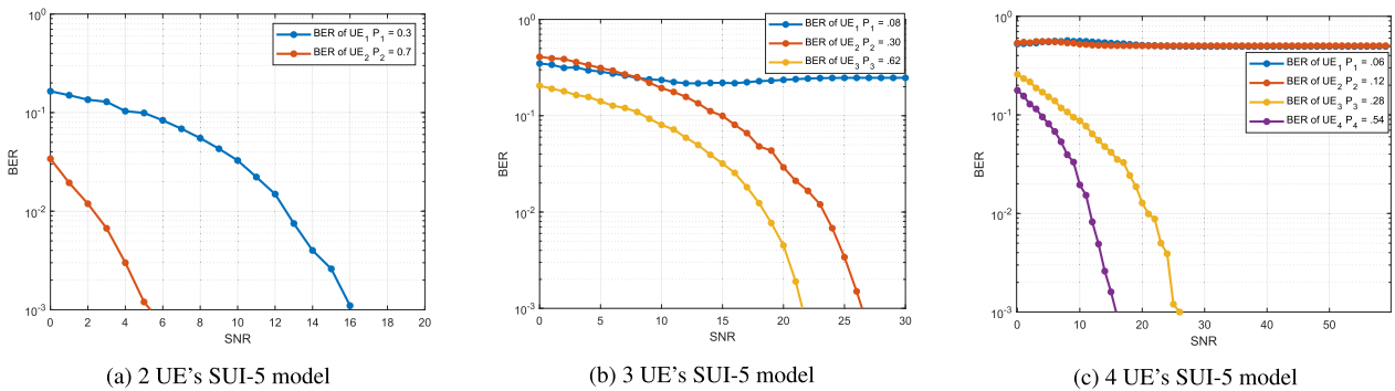
FIGURE 9. BER performance of 2, 3 and 4 UE's per cluster PD-NOMA system under SUI-5 channel model.
