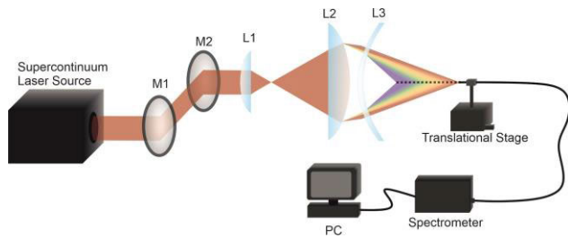
FIGURE 2. Experimental set-up for hyperspectral imaging source generation. Mirror (M1, M2), Lens (L1, L2, L3), Personal computer (PC).
