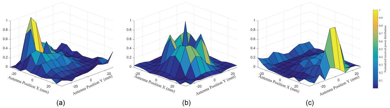
FIGURE 5. Normalized received power distribution of all antenna elements in the case of normal incidence (a) \theta = 35^\circ , \phi = 241.9^\circ , (b) \theta = 0^\circ , \phi = 0^\circ , and (c) \theta = 30^\circ , \phi = 78.8^\circ .
