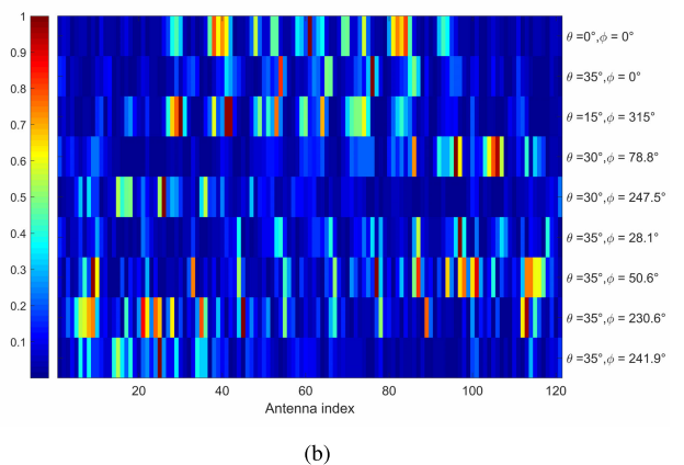
FIGURE 3. Normalized received power distribution on the proposed lens antenna array for vertically polarized plane waves with different AoAs: (a) received power curves; (b) power image where the intensity is represented by colored pixels.
