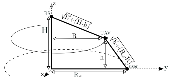
FIGURE 5. Scheme of three DOF and two DOF trajectory for one UAV. The variables are R (trajectory radius), h (trajectory plane height) and V (UAV velocity).
