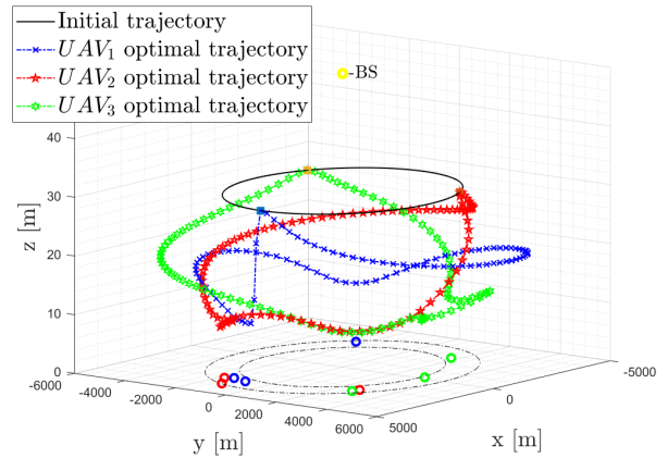
FIGURE 6. Optimized trajectory for unbounded 3D trajectory.
