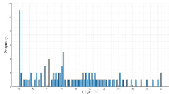
FIGURE 7. For the third UAV of the 3D optimized trajectory are classified the heights.
