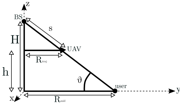
FIGURE 4. A trigonometrical representation of a cone constrained trajectory optimization for one UAV.
