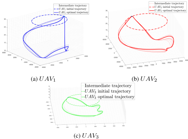
FIGURE 9. 3D Trajectory Evolution for the trajectories shown in Figure 6.
