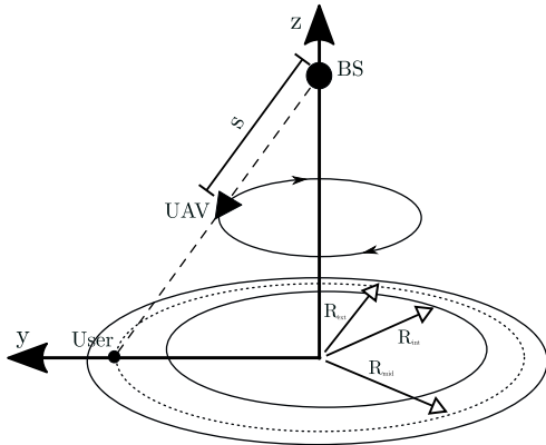
FIGURE 3. Scheme of cone constrained trajectory optimization for one UAV. In this scenario, the geometry is much simplified.
