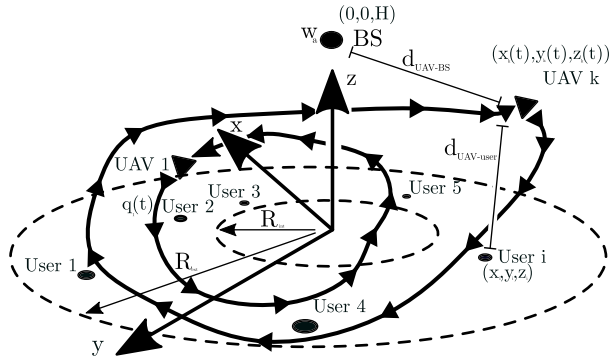
FIGURE 2. Sample UAVs' trajectory scheme of the system. It is shown the GTs (ground terminals) positions and the UAVs' trajectory.
