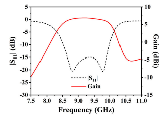
FIGURE 5. Simulated |S_{11}| and gain of basic antenna without the NZIM and balun.
