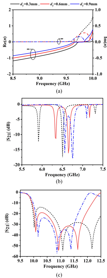
FIGURE 10. The simulated results of the NZIM array, (a) Refractive index n , (b) transmission coefficient ( |S_{21}| ) in the lower notch band, and (c) |S_{21}| in the upper notch band under different d_y .
