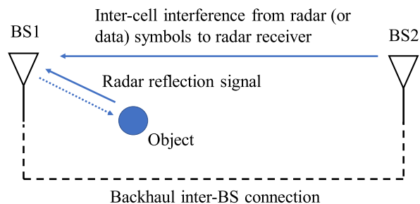
FIGURE 7. Radar-to-radar inter-cell interference cancellation.
