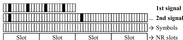
FIGURE 6. Pair of signals for low-overhead radar excitation.
