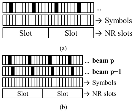
FIGURE 4. a. Time interleaved signal allocation for a particular beam. Black: Sensing, White: Communication data. b. Time interleaved signal allocation for two beams.
