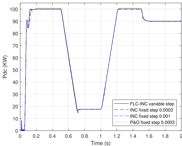
FIGURE 17. The comparison of output dc power when applying the conventional INC and the conventional P&O MPPT methods when using fixed step size and that of the FLC based variable step size for ramp variations of G and T_c .
