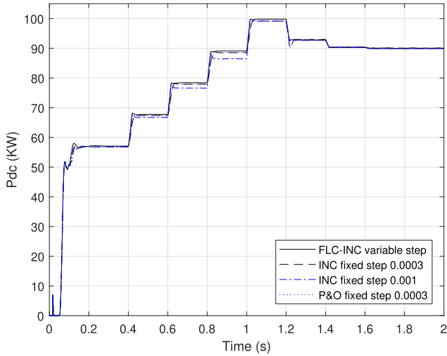
FIGURE 13. The output dc power comparison when applying the conventional fixed step INC method, the fixed step P&O method and the FLC based variable step INC method for MPPT.
