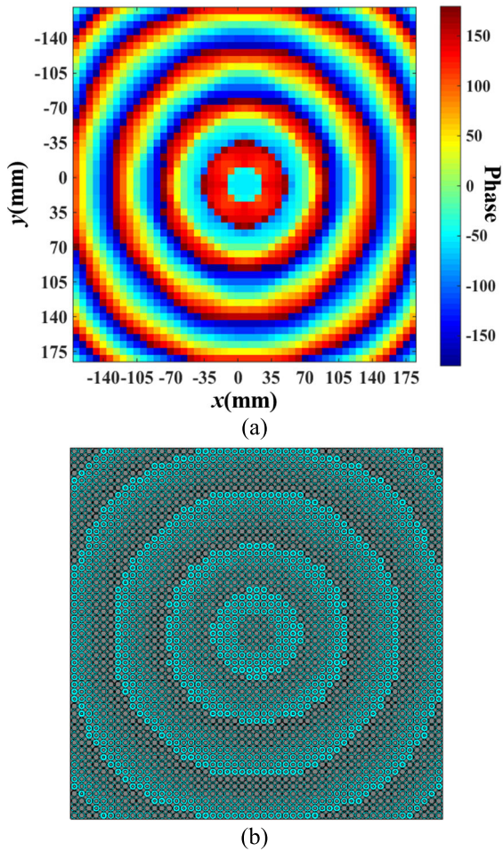
FIGURE 5. (a) Phase distribution of TR Bessel beam and (b) TR Bessel lens structure.
