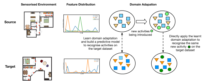
FIGURE 1. A use case [17] of generalised unsupervised domain adaptation.
