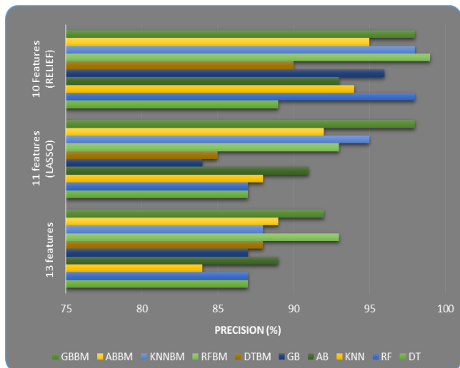
FIGURE 11. Precision.
