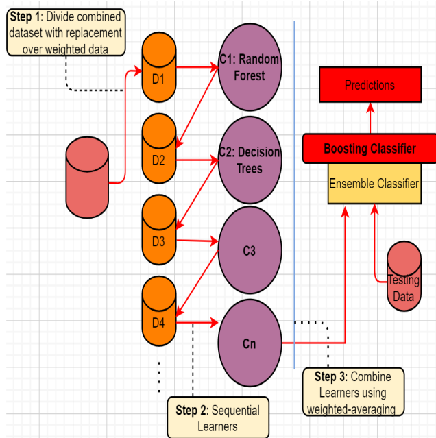
FIGURE 7. Boosting method.
