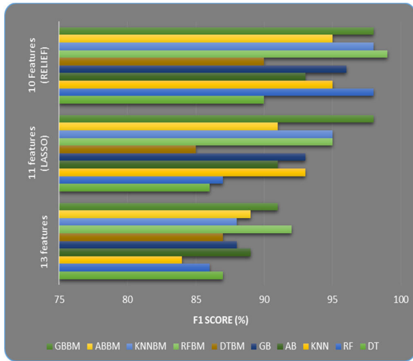
FIGURE 13. Obtained F1-scores.
