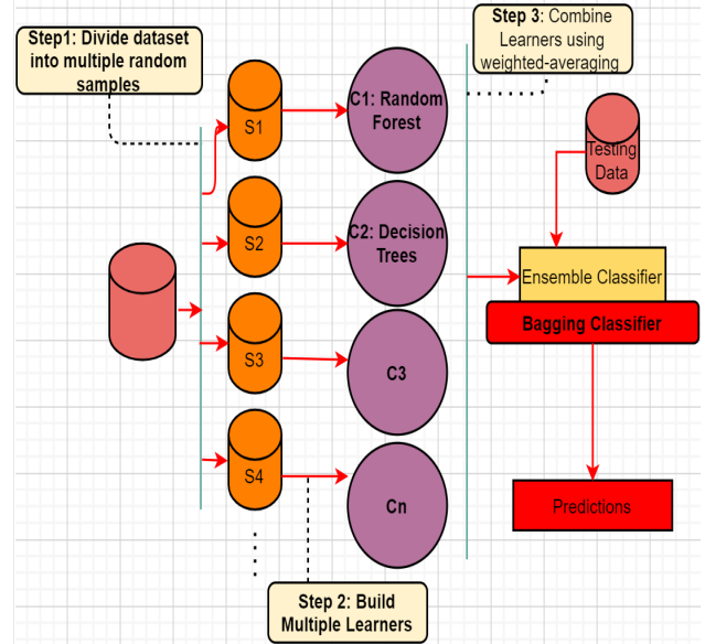
FIGURE 6. Bagging method.
