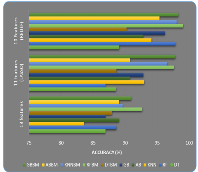
FIGURE 9. Accuracy.
