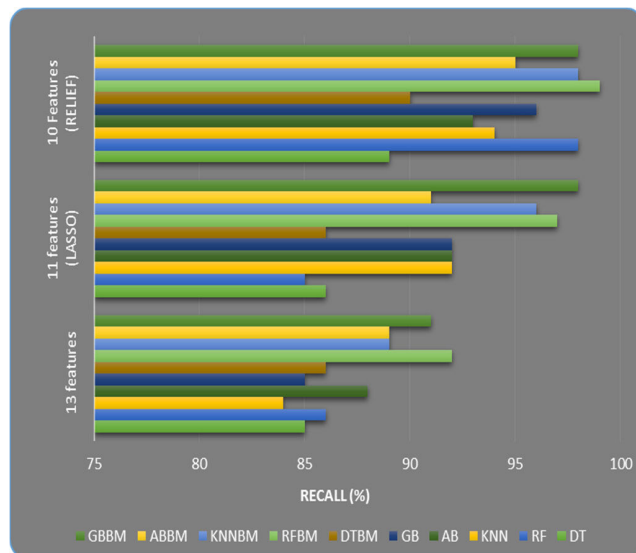
FIGURE 12. Obtained recall scores.
