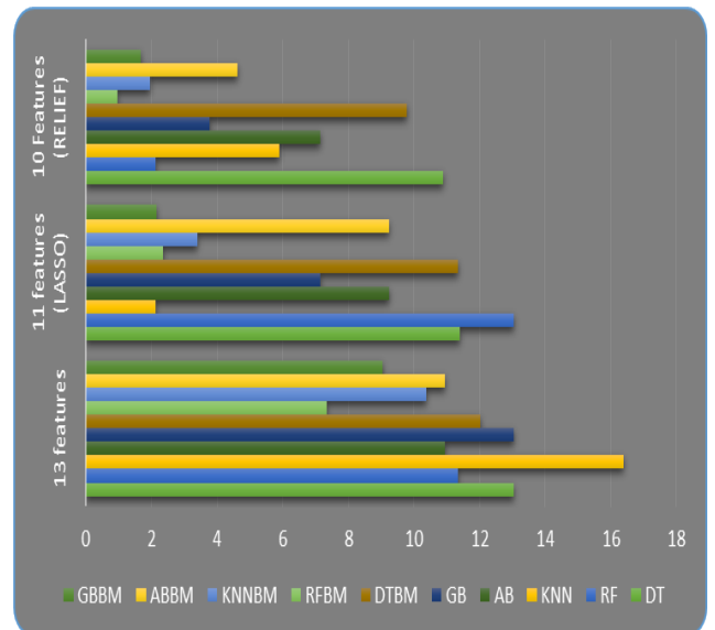
FIGURE 10. Error rates.
