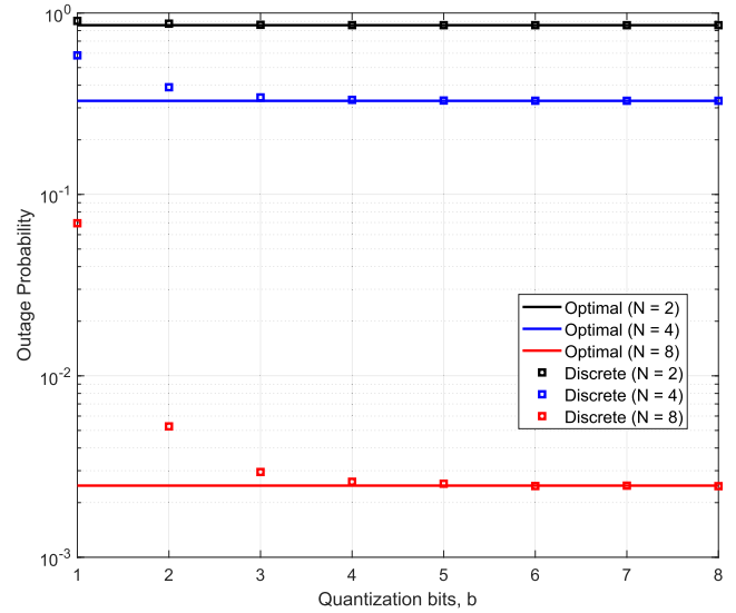
FIGURE 14. Outage probability versus number of quantization bits, b , for different values of N .
