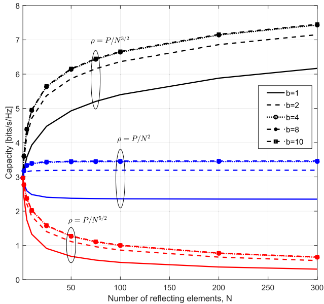
FIGURE 8. Power scaling law for different \alpha values.
