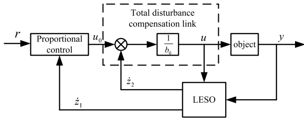
FIGURE 4. LADRC control block diagram.
