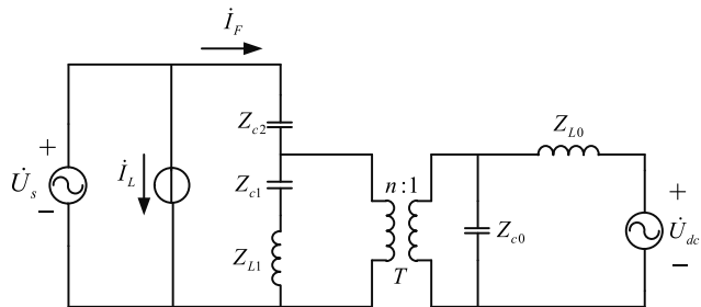
FIGURE 2. IHAPF single phase equivalent circuit.
