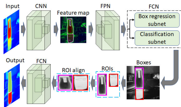
FIGURE 6. Architecture of Mask R-CNN.
