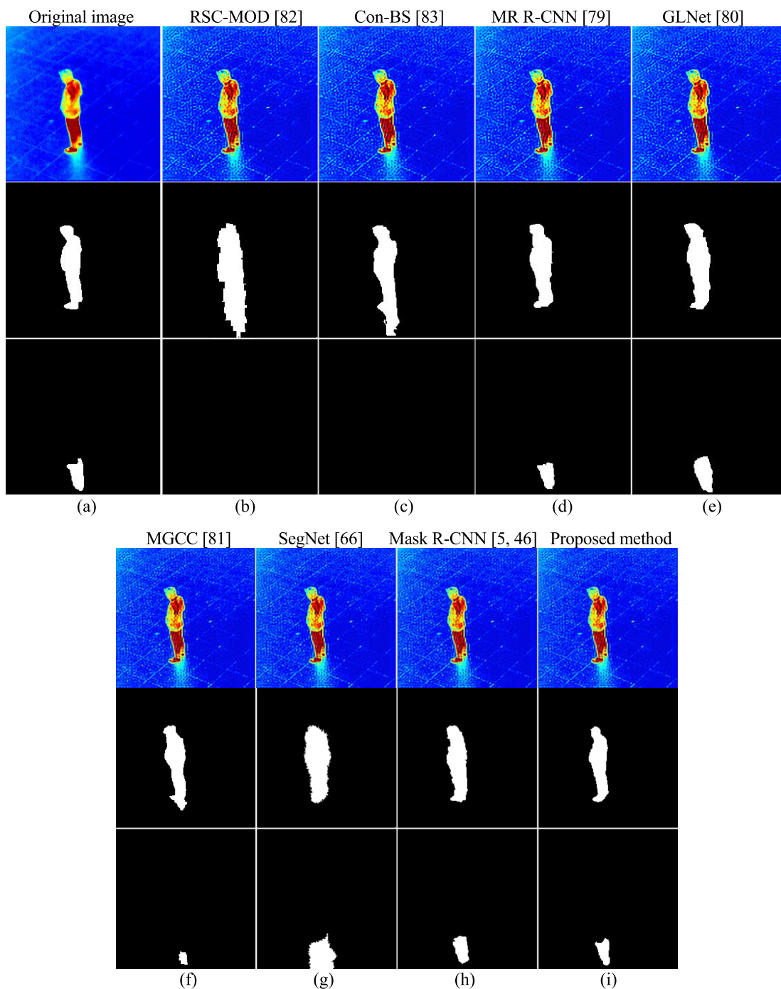
FIGURE 15. Examples of detection results using restored images (upsampling factor = 2 and kernel size = 13 \times 13 ). From the top to the bottom, input images, detected results of an object, and a thermal reflection. (a) ground truth masks; (b) result mask images by RSC-MOD [82]; (c) result mask images by Con-BS [83]; (d) result mask images by MR R-CNN [79]; (e) result mask images by GLNet [80]; (f) result mask images by MGCC [81]; (g) result mask images by SegNet [66]; (h) result mask images by Mask R-CNN [5], [46]; (i) result mask images by proposed method.
