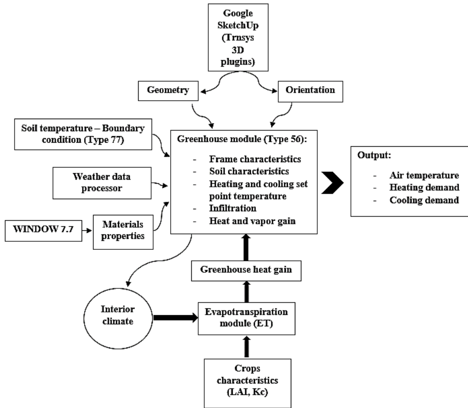
FIGURE 2. Diagram of this greenhouse model on TRNSYS.
