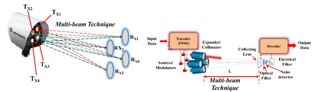
FIGURE 3. Multi-beam FSO system [7].
