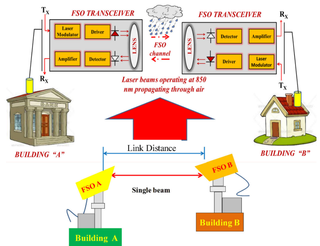
FIGURE 2. Overview of single beam FSO communication system in static placement [18].
