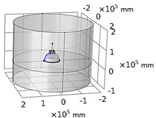
FIGURE 15. Typical COMSOL layout for monument for analysis of lightning-human interaction mechanisms.
