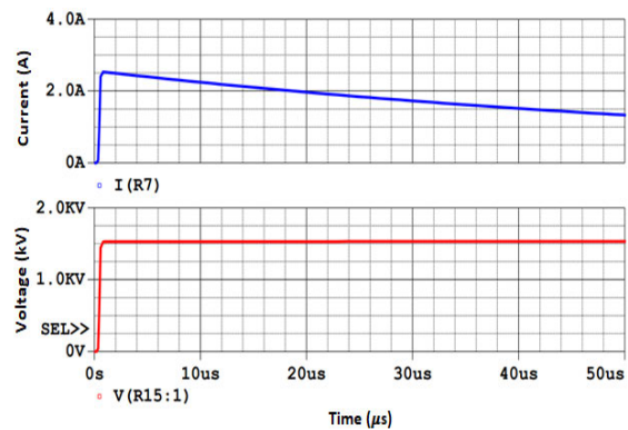
FIGURE 37. Step voltage and leg current waveforms of lightning flash at a distance of 1.5m from the monument with 5 Ω earthing resistance.
