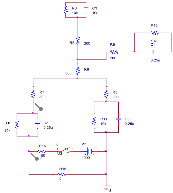
FIGURE 34. Simulation of human step potential due to direct strike to the LPS of the monuments (with 5 \Omega earthing resistance).
