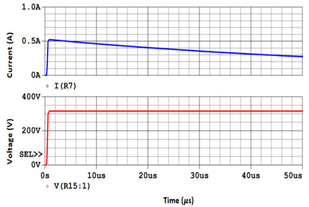
FIGURE 38. Step voltage and leg current waveforms of lightning flash at a distance of 1.5m from the monument with 1 Ω earthing resistance.
