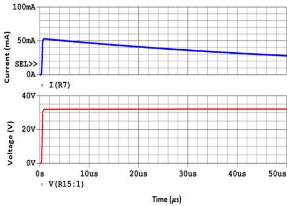
FIGURE 35. Step voltage and leg current waveforms of lightning flash at a distance of 10m from the monument with 5 Ω earthing resistance.
