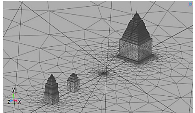
FIGURE 20. FEM meshing diagram for Big Temple.
