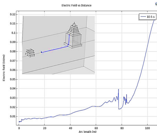
FIGURE 29. Electric field distribution during strike on Gangaikonda Cholapuram.
