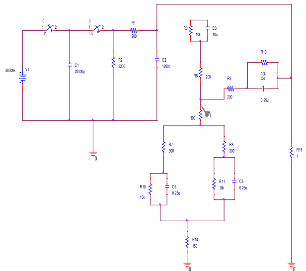
FIGURE 39. Simulation of human touch potential and current due to direct strike to the LPS of the monuments (with 1 Ω earthing resistance).
