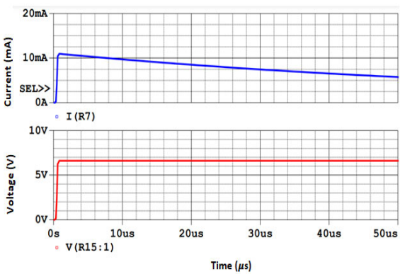
FIGURE 36. Step voltage and leg current waveforms of lightning flash at a distance of 10m from the monument with 1 Ω earthing resistance.
