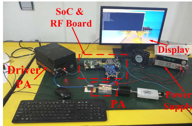
FIGURE 9. Experimental setup.
