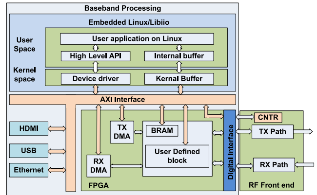
FIGURE 6. Interfacing between PSU and PLU.
