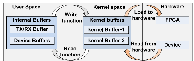
FIGURE 7. Buffer structure.
