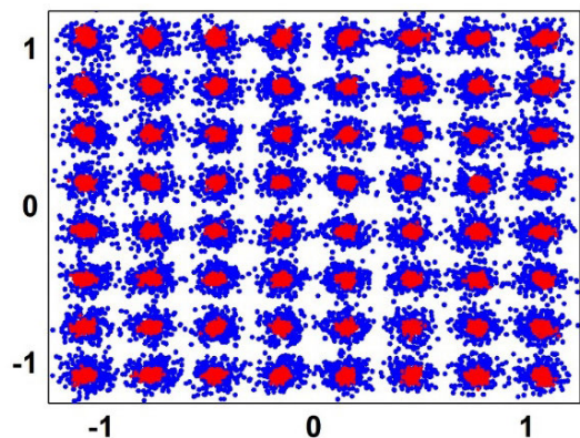
FIGURE 15. Constellation Plot of 20 MHz LTE signal at PA output without DPD (BLUE) and with DPD (RED).
