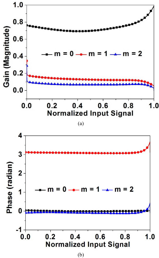
FIGURE 11. Calculated inverse gain values G_{inv} and (b) inverse phase values \Phi_{inv} for m = 0, 1, 2 to generate a predistorted signal.
