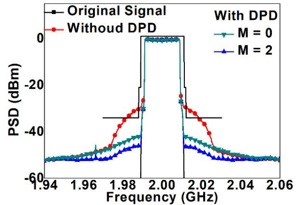
FIGURE 12. ADPD performance with and without Memory effect using 20 MHz LTE signal.
