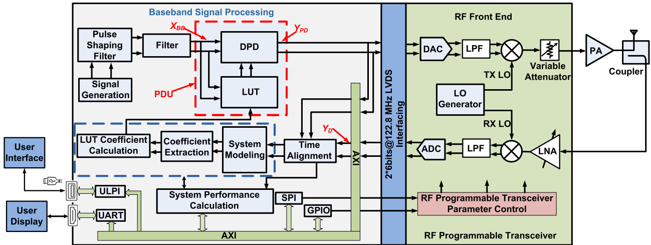
FIGURE 3. Proposed SDR transceiver architecture with adaptive DPD solution.
