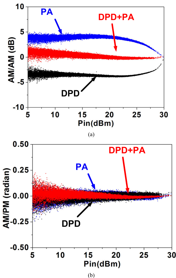
FIGURE 13. (a) AM/AM. (b) AM/PM characteristics at PA output with and without using ADPD.
