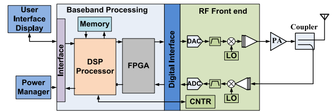
FIGURE 2. SDR based transmitter architecture.
