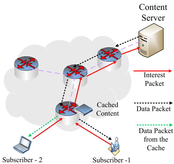
FIGURE 3. Caching in an ICN.
