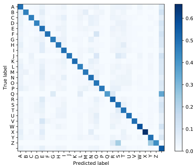
FIGURE 13. Confusion matrix for classification of ASCII characters.
