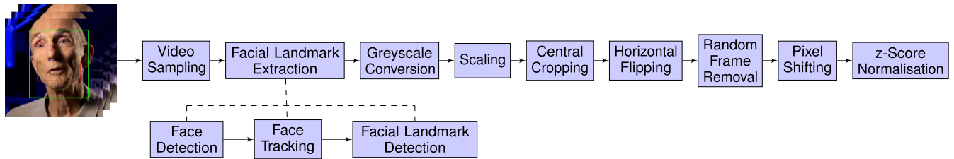
FIGURE 4. The stages of video image pre-processing.
