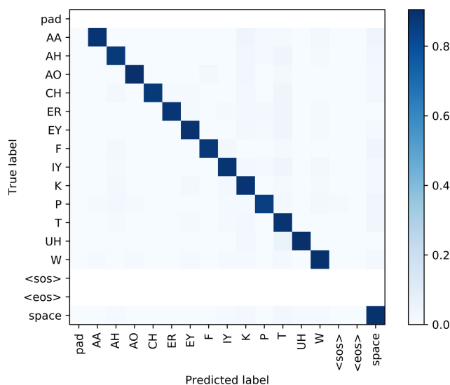
FIGURE 12. Confusion matrix for classification of visemes.
