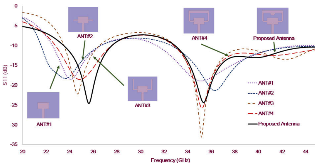
FIGURE 4. S11 of the antenna evolution.
