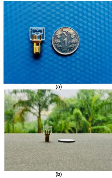
FIGURE 2. Fabricated Single Element Transparent Antenna (a) Top View (b) Front View.
