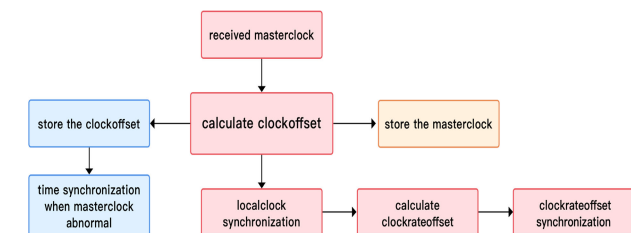
FIGURE 4. Behavior of the slave clock node.
