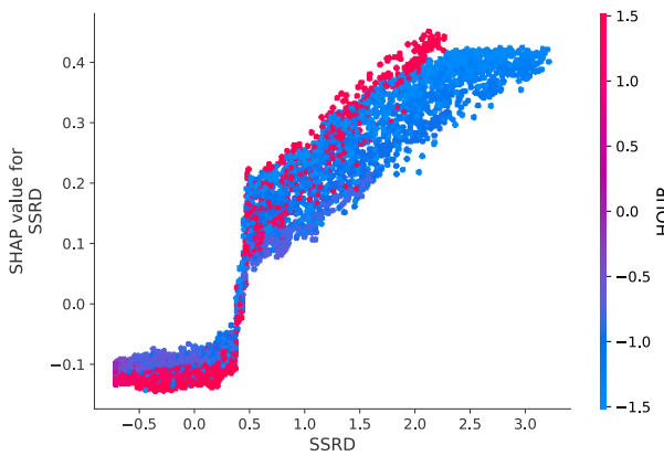
FIGURE 8. Dependence plot of SSRD.
