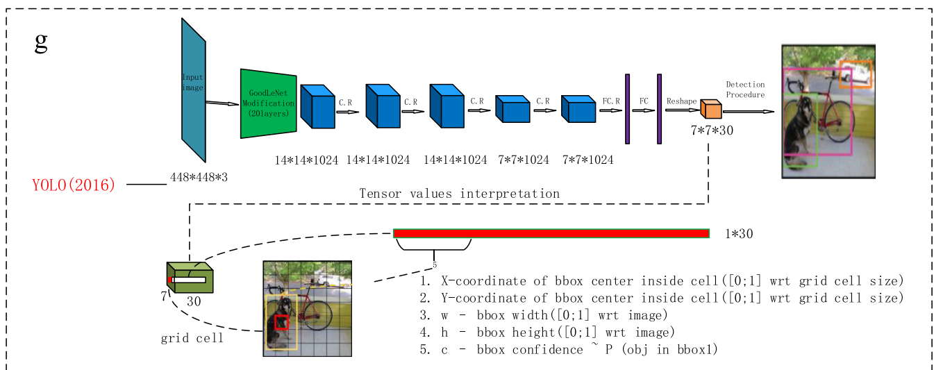
FIGURE 2. (Continued.) Development track of machine vision based on CNNs. (a) LeNet-5 [84]. (b) AlexNet-5 [22]. (c) GoogLeNet [87]. (d) VGG-16 [92]. (e) Faster-RCNN [94]. (f) ResNet [97]. (g) YOLO [103]. (h) SSD [100]. (i) YOLOv3 [119]. (j) RetinaNet [111]. (k) CornerNet [112].
