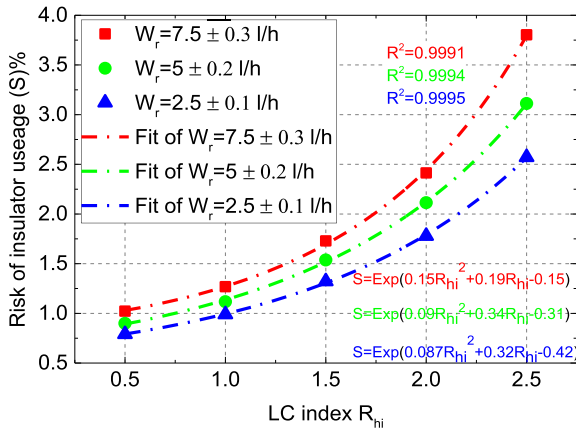
FIGURE 18. Risk of insulator string type A utilization as a function of LC index in different of wetting rate W_r , j = 1 and z = 1/3 .
