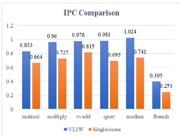
FIGURE 11. IPC comparison between the VLIW and single-issue core.
