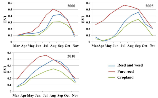
FIGURE 3. EVI series of three land cover classes in 2000, 2005 and 2010.
