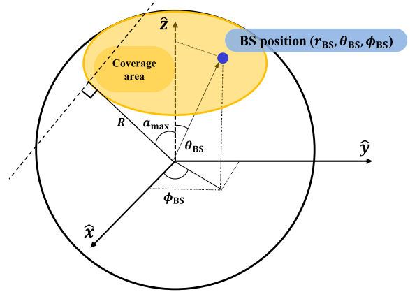
a) Spherical coordinates of distributed BS
