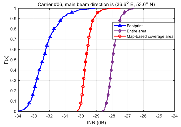
(a) Carrier #06, Main beam direction: (36.6^\circ \text{ E}, 53.6^\circ \text{ N})
