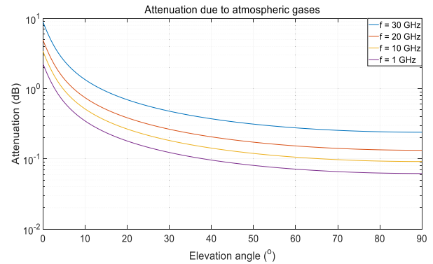
FIGURE 10. Attenuation by atmospheric gases.
