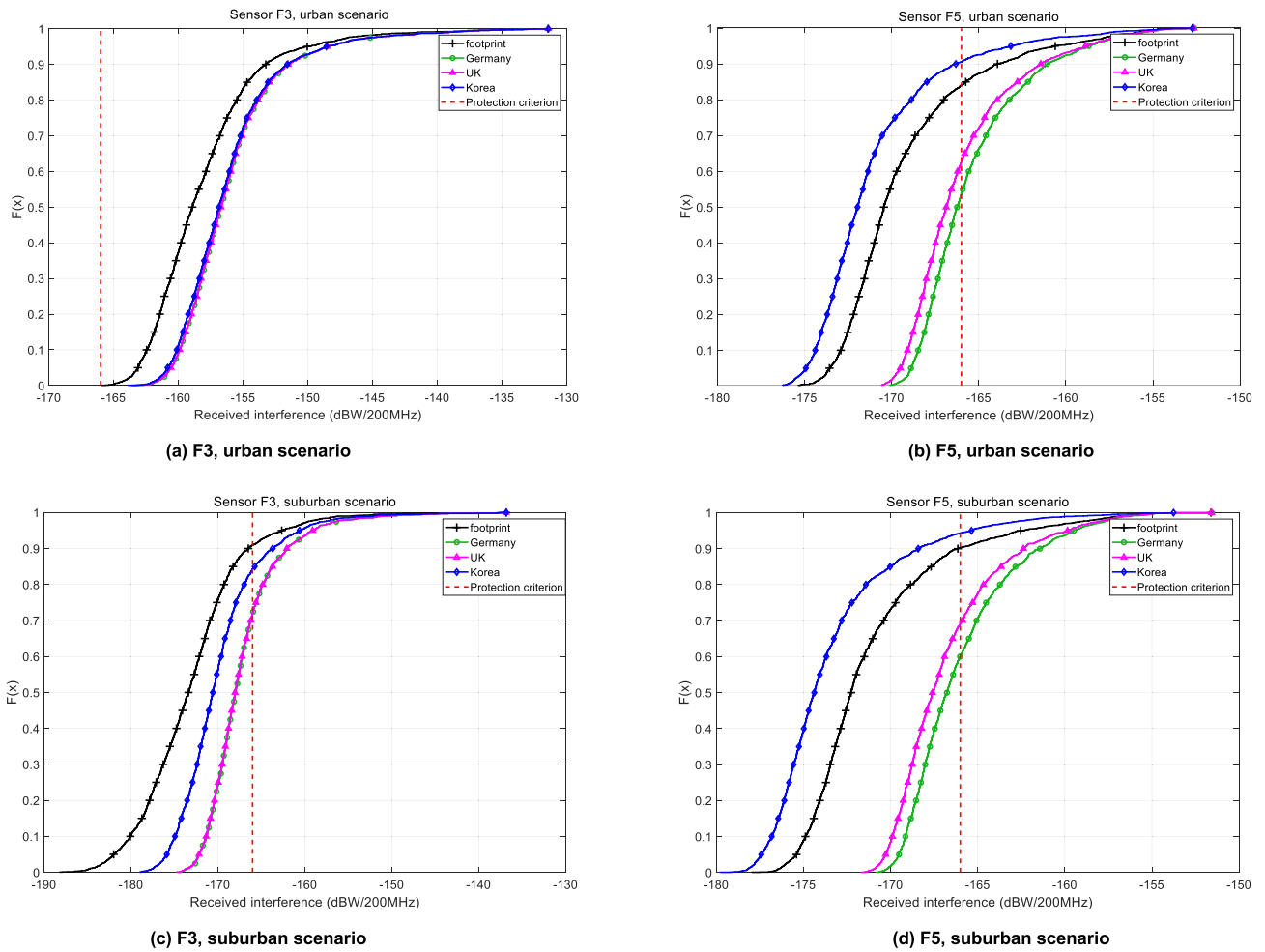
FIGURE 20. CDF of received interference power of the EESS passive sensors. (BS: 16 × 16, UE: 8 × 8).
