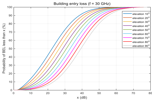
FIGURE 9. Building entry loss ( f = 30 GHz).
