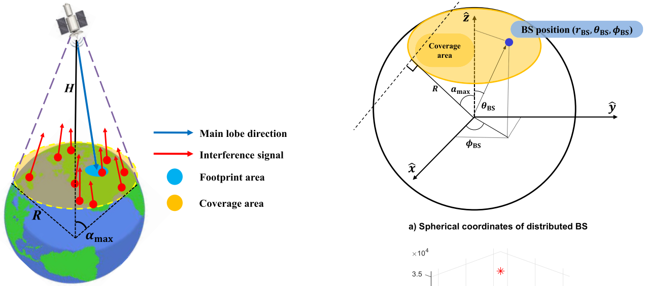
FIGURE 1. Interference scenario that satellite receives from IMT-2020.
