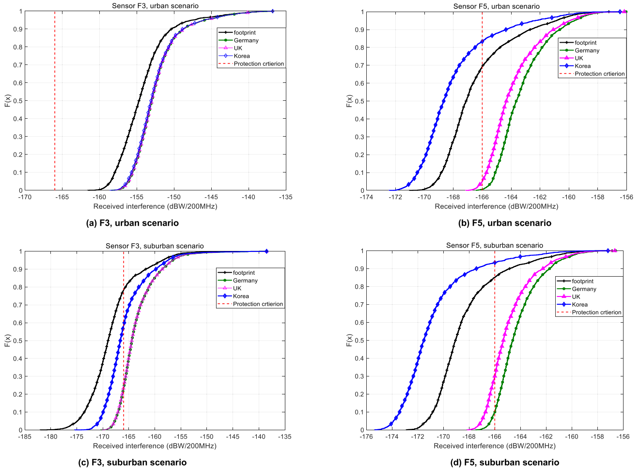
FIGURE 19. CDF of received interference power of the EESS passive sensors. (BS: 8 × 8, UE: 4 × 4).
