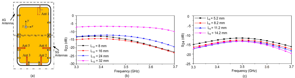
FIGURE 13. Multiband metal rim 5G MIMO antenna [148] (a) A single ring slot based antennas for metal rim 4G/5G smartphones. (b) Mutual coupling between Ant 2 and Ant 3 for different values of L12 (c) Mutual coupling between Ant 2 and Ant 4 for different values of L9.
