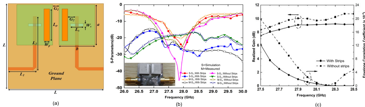
FIGURE 7. Dielectric resonator antenna design [84] (a) Top view of MIMO DRA (b) S parameters (c) Gain and ECC.
