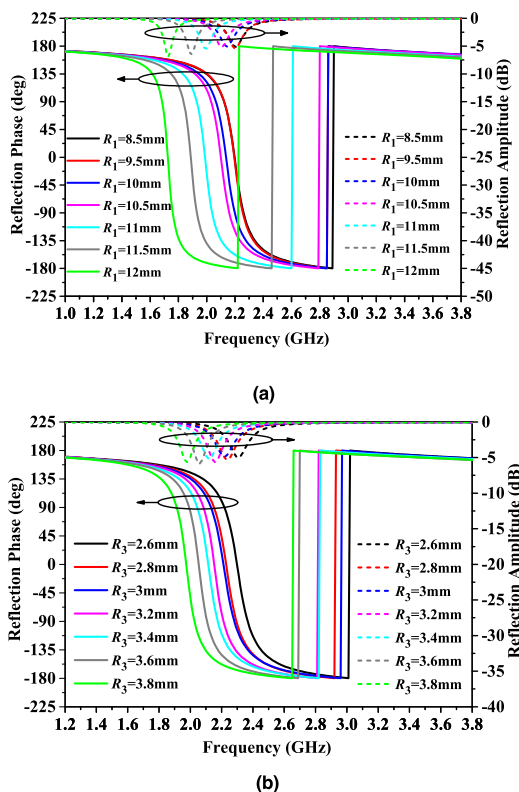
FIGURE 3. The reflection coefficients of the CFRN-AMC in the cases of (a) R_1 = 8.5 \sim 12 mm, and (b) R_3 = 2.6 \sim 3.8 mm.
