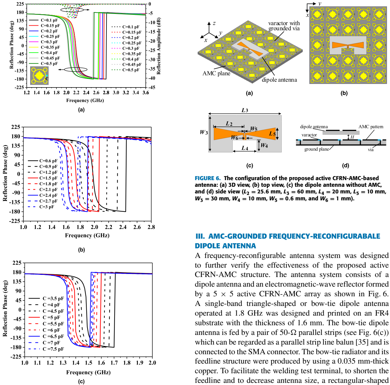
FIGURE 5. The phases of the reflection coefficients for the active CFRN-AMC with the capacitance in the cases of (a) 0.1~0.5 pF, (b) 0.6~3 pF, and (c) 3.5~7.5 pF.
