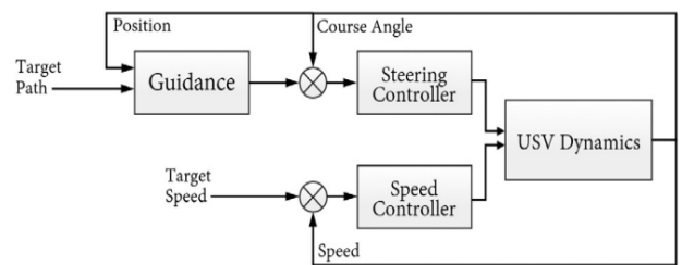
FIGURE 5. Block diagram from the unmanned surface vehicle path following system [40].
