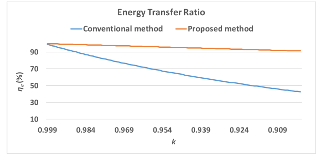
FIGURE 4. Energy transfer ratio in flyback operation
