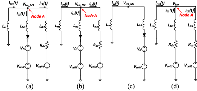
FIGURE 3. Equivalent circuit diagram of the balancing circuit in flyback operation: (a) Mode 3 in the conventional method, (b), (c) Mode 2, 3 in the proposed method, (d) S_1 and S_3 are turned on simultaneously in the proposed method.
