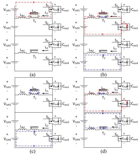
FIGURE 1. Current path of cell balancing circuit in flyback operation: (a) ~ (c) Mode 1, 3, and 4 in the conventional method, (d) Mode 2 in the proposed method.
