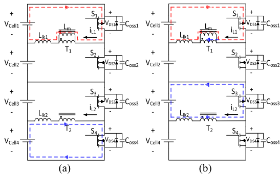
FIGURE 5. Current paths of cell balancing circuit in the proposed forward operation: (a) Mode 1, (b) Mode 3.
