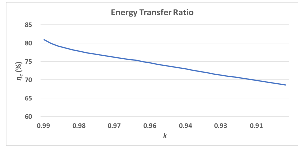
FIGURE 8. Energy transfer ratio in the proposed forward operation according to the coupling coefficient.
