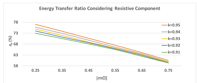
FIGURE 9. Energy transfer ratio in the proposed forward operation considering different resistance component.
