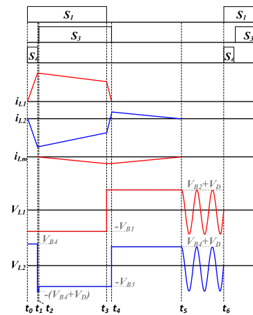
FIGURE 7. Theoretical waveforms of the proposed forward operation.
