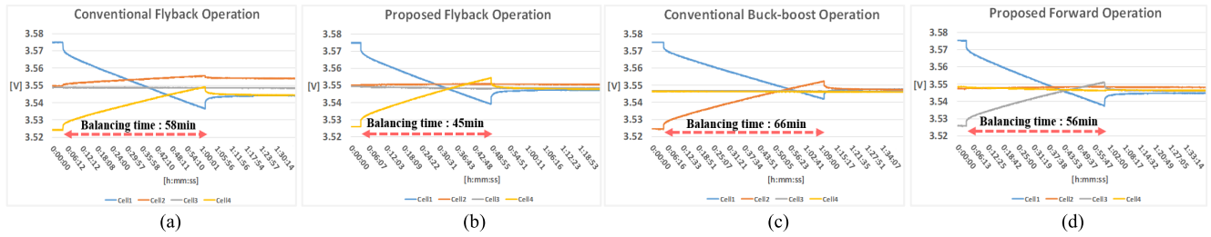
FIGURE 14. Balancing speed of cell voltage according to operational methods: (a) Conventional flyback operation, (b) Proposed flyback operation, (c) Conventional buck-boost operation, (d) Proposed forward operation.
