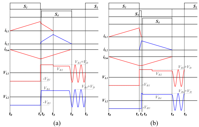
FIGURE 2. Theoretical waveforms of the conventional flyback operation: (a) Conventional flyback operation, (b) Proposed flyback operation.
