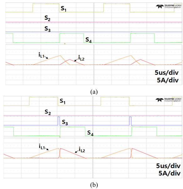
FIGURE 12. Experimental waveforms ( k = 0.92 ): (a) Switching signals and current waveforms in the conventional flyback operation (5us/div) (b) Switching signals and current waveforms in the proposed flyback operation (5us/div).
