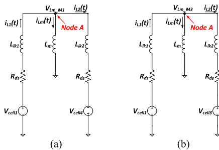
FIGURE 6. Equivalent circuit diagram of cell balancing circuit in the proposed forward operation: (a) Mode 1, (b) Mode 3.
