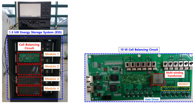
FIGURE 10. 12-cell series connected 15 W prototype cell balancing circuit.
