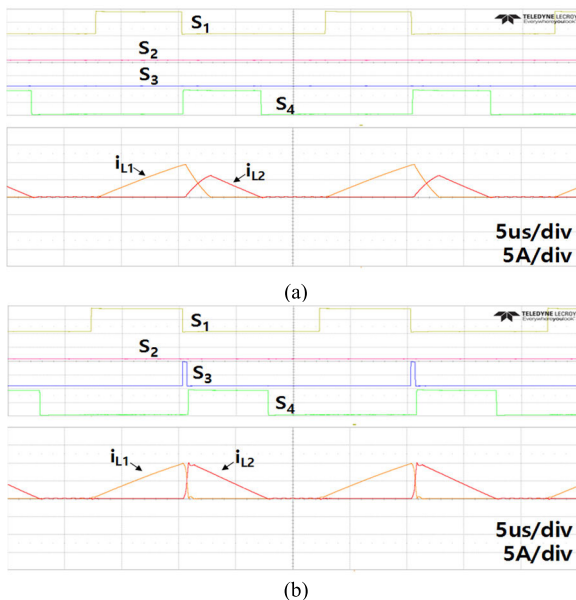
FIGURE 11. Experimental waveforms ( k = 0.948 ): (a) Switching signals and current waveforms in the conventional flyback operation (5us/div) (b) Switching signals and current waveforms in the proposed flyback operation (5us/div).
