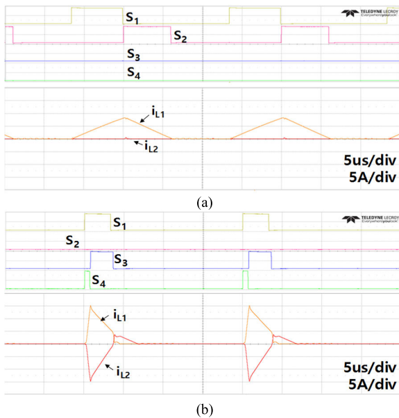
FIGURE 13. Experimental waveforms ( k = 0.948 ): (a) Switching signals and current waveforms in the conventional buck-boost operation (5us/div), (b) Switching signals and current waveforms in the proposed forward operation (5us/div).
