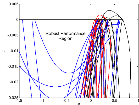
FIGURE 8. Robust performance region for the interval plant (17), (18).
