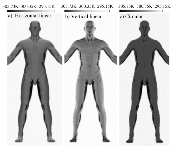
FIGURE 6. Scene simulation of an image of a person at 20 GHz illustrating the effects in a) horizontal linear, b) vertical linear and c) circular polarization. The Brewster angle reflection and body canyon illumination effects can be observed. The radiometric temperature is on the scale above the image; black represents radiometrically ‘hot’.
