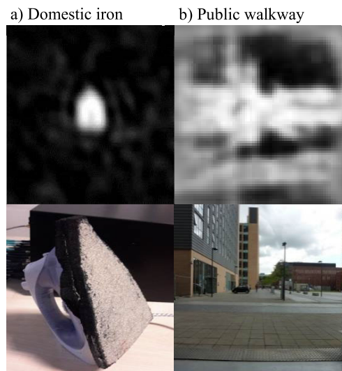
FIGURE 2. Images measured using a 32-channel 22 GHz aperture synthesis imager of: a) an absorber covered domestic iron at 57°C against an ambient temperature (23°C) background [22] b) an outdoor public walkway [20], white being radiometrically ‘hot’
