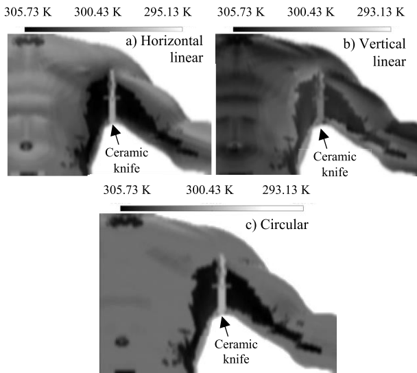
FIGURE 9. The simulated image of the ceramic knife in the armpit showing (clockwise from the top left) the effects in a) horizontal linear, b) vertical linear and c) circular polarization. Circular polarization offers the least clutter due to the absence of Brewster angle effects.
